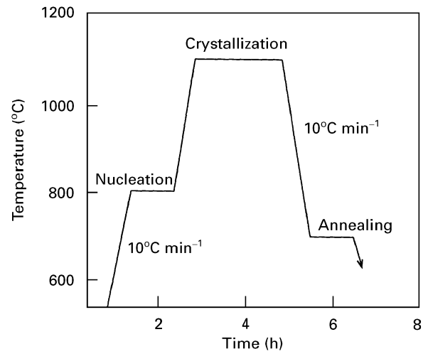
Figure 4 Heat-treatment schedule.
